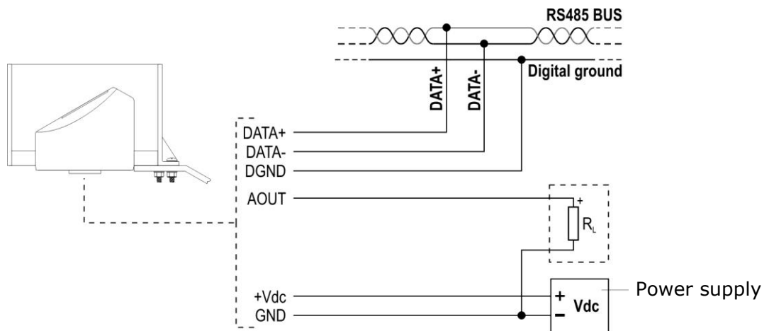
Fig. 3.3: connections
