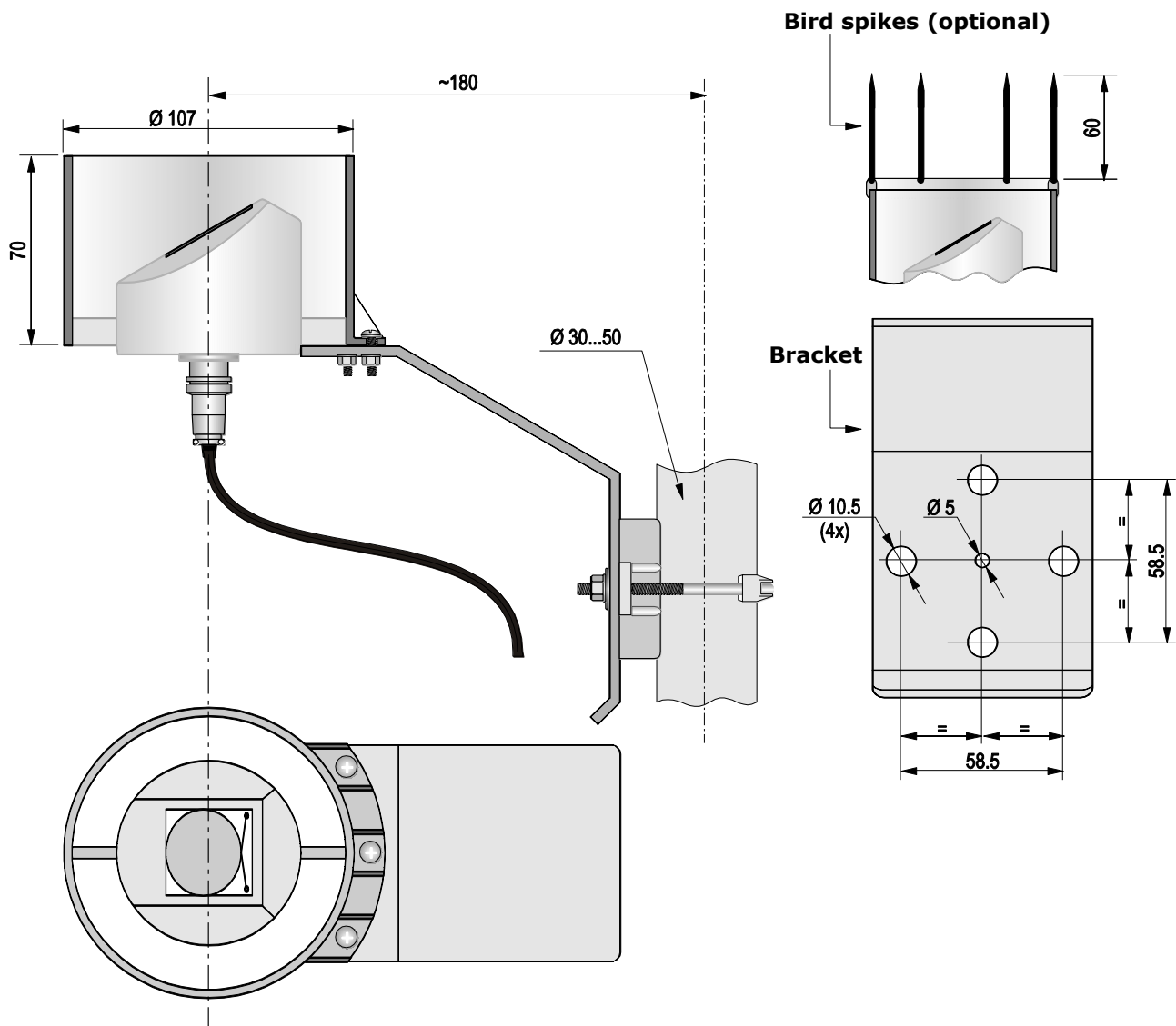
Fig. 2.1: dimensions (mm)
