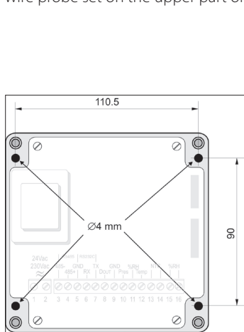
Position of the fixing holes
