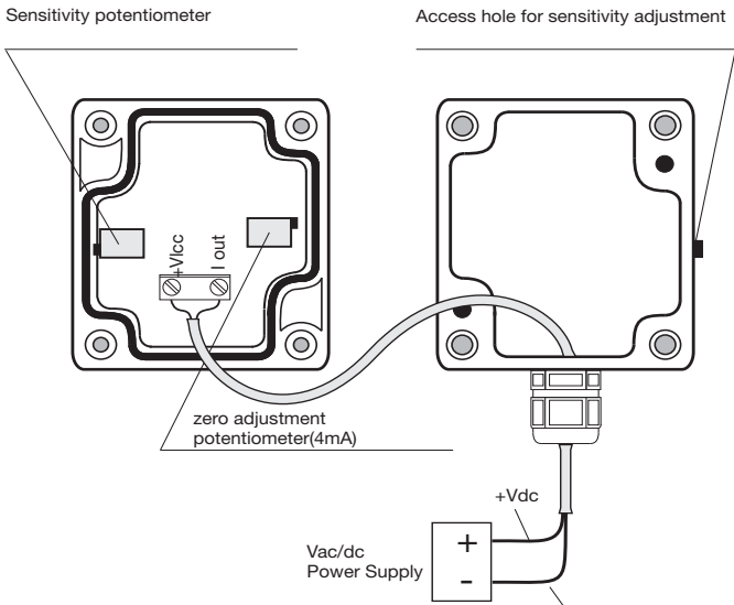
Figure 5 - Connection diagram for HD2021T... with current output
