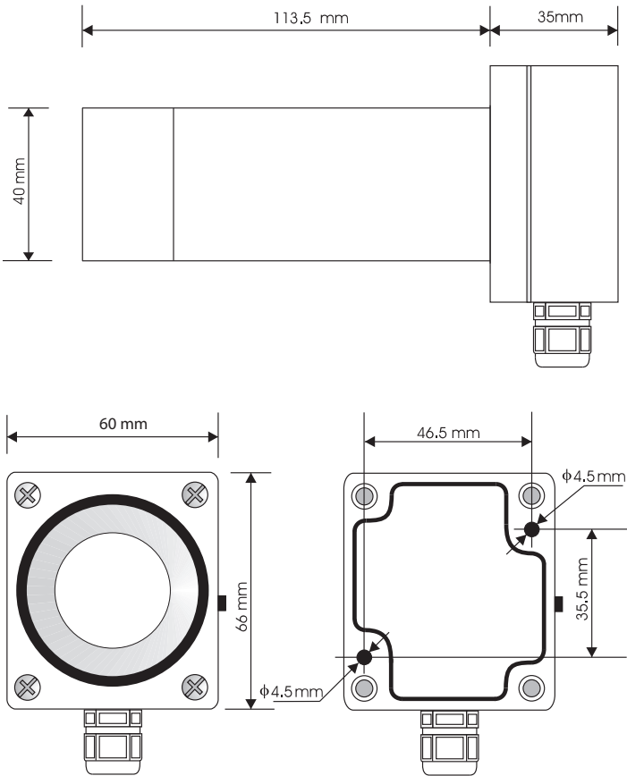
Figure 6 - HD2021T6 probe dimensions
