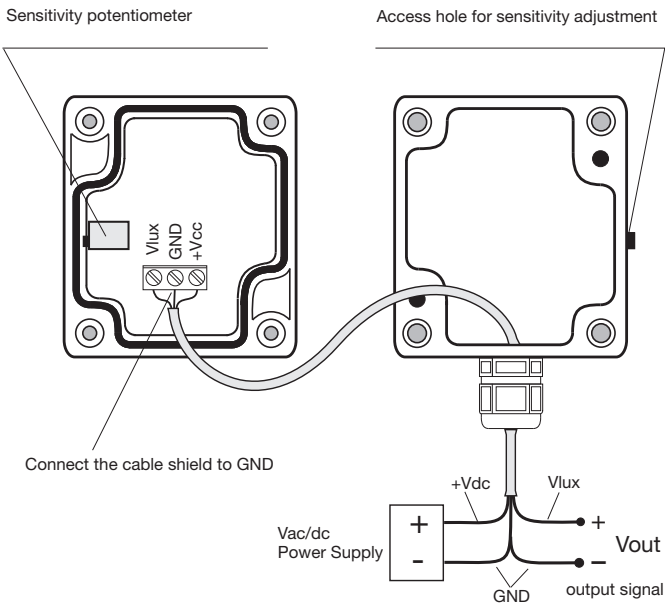
Figure 4 - Connection diagram for HD2021T... with voltage output
