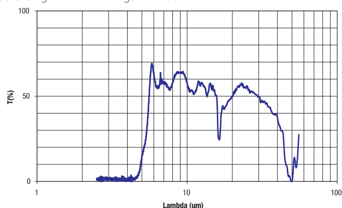
Graph 2 - Transmission of the silicon window.
